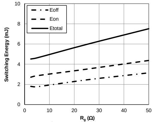
Figure 18: Switching Loss vs. R_g ( T_J=175^\circ\text{C} , V_{GE}=15\text{V} , V_{CE}=400\text{V} , I_C=60\text{A} )
