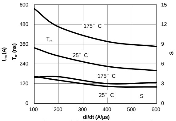
Figure 24: Diode Reverse Recovery Time and Softness Factor vs. di/dt ( V_{GE}=15V , V_{CE}=400V , I_F=60A )
