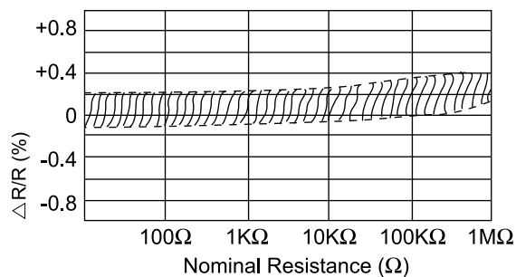
Load Life
