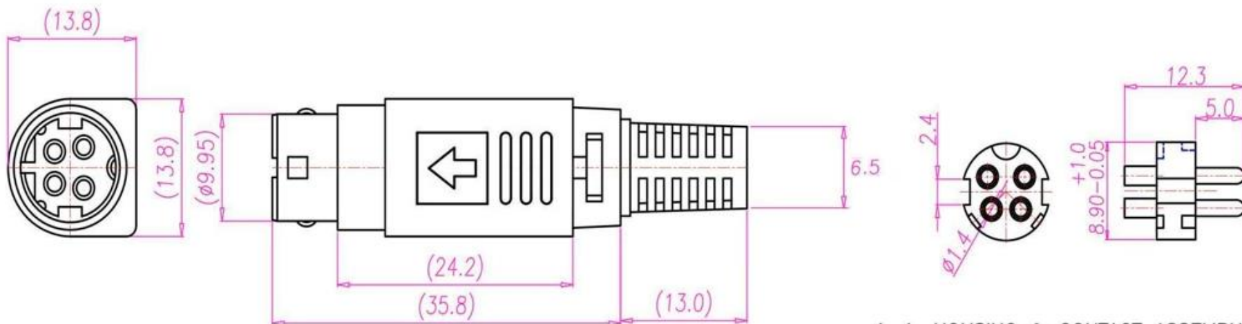
1-1. HOUSING & CONTACT ASSEMBLY
