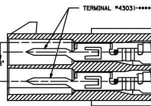
SECTION "D"- "D" WITH TERMINAL (SCALE 8X)
