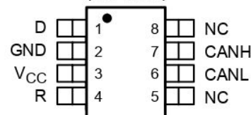
SN65HVD232D (Marked as VP232) (TOP VIEW)
