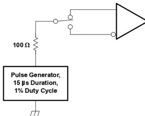
Figure 7. Overvoltage Protection
