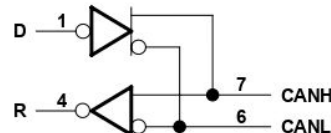
SN65HVD232 Logic Diagram (Positive Logic)
