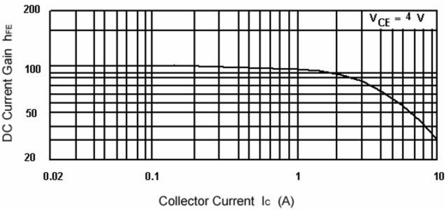
Fig.5 DC current Gain
