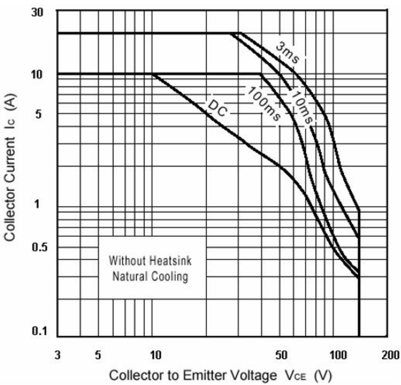
Fig.4 Safe Operating Area
