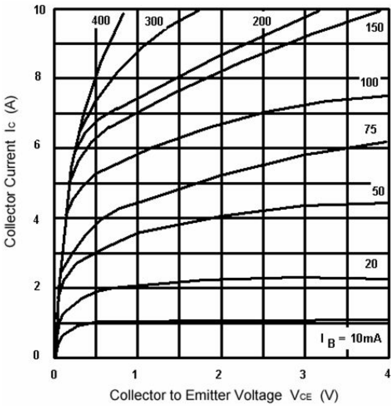
Fig.3 Static Characteristic
