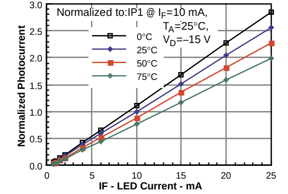
Figure 6. Normalized servo photocurrent vs. LED current and temperature
