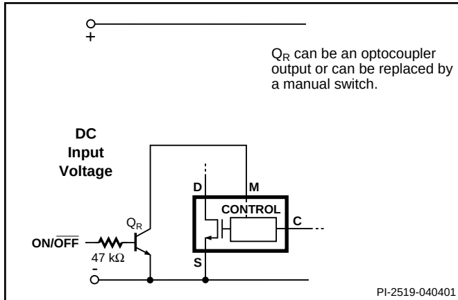
Figure 19. Active-on (Fail Safe) Remote ON/OFF.
