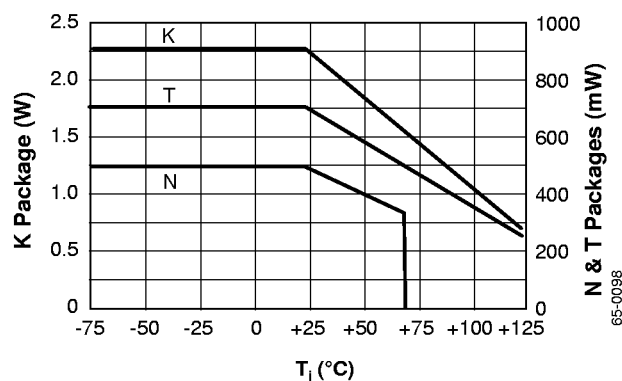
Figure 4. Power Dissipation
