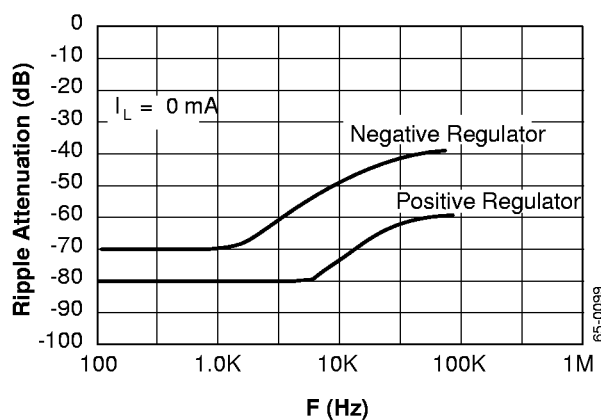
Figure 6. Ripple Rejection
