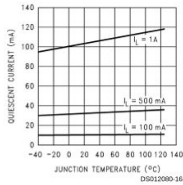
Quiescent Current vs Temperature
