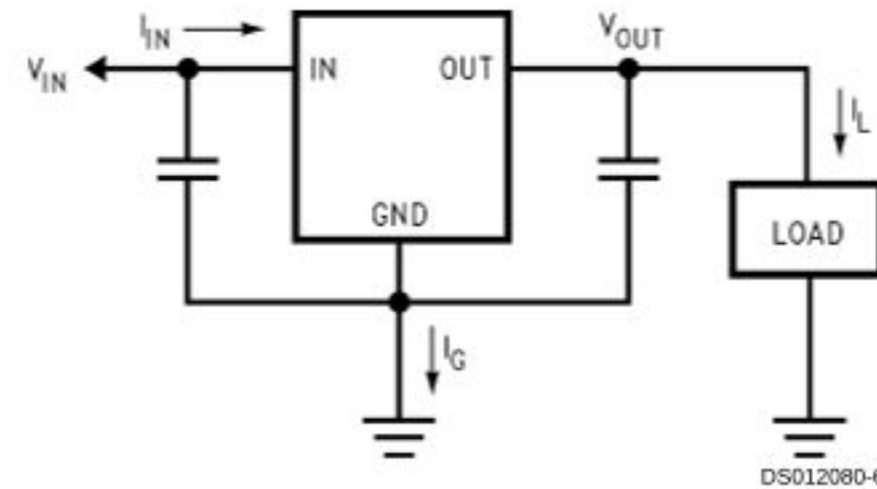
FIGURE 2. Power Dissipation Diagram
