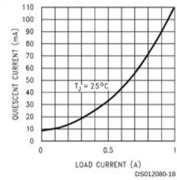
Quiescent Current vs Load
