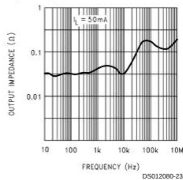
Output Impedance
