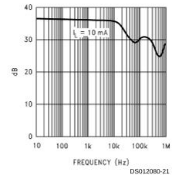
Ripple Rejection
