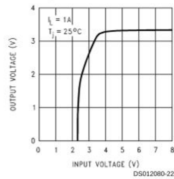
Low Voltage Behavior
