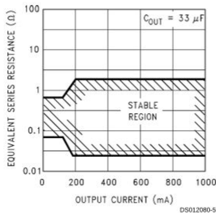
FIGURE 1. ESR Limits
