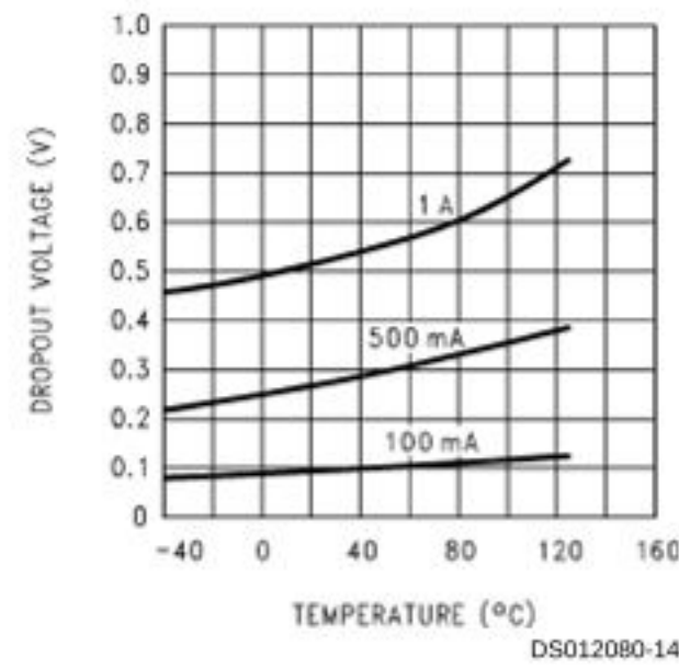
Dropout Voltage vs Temperature
