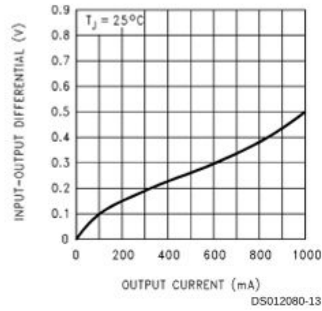
Dropout Voltage
