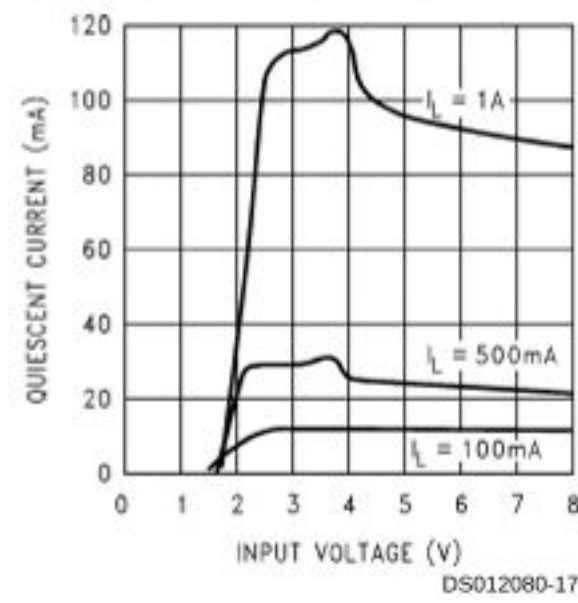
Quiescent Current vs V_{IN}
