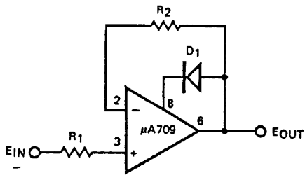
LATCH-UP PROTECTION
