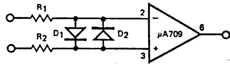
INPUT BREAKDOWN-PROTECTION
