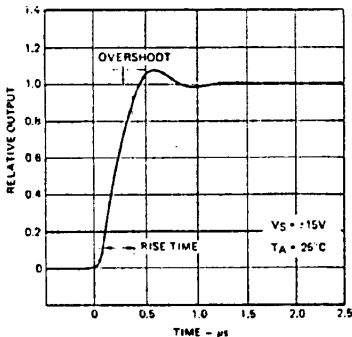
TRANSIENT RESPONSE
