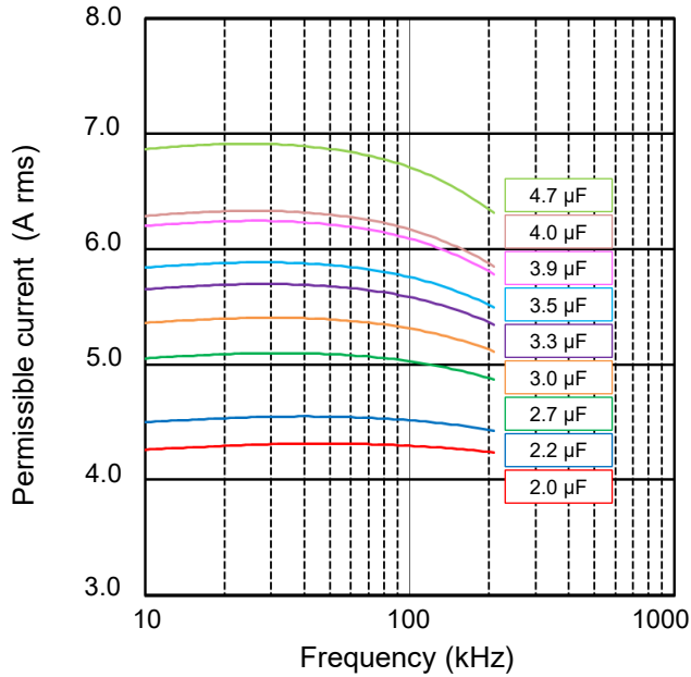
[ Permissible Current ]
