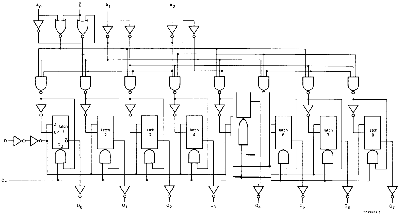
Fig.3 Logic diagram.
