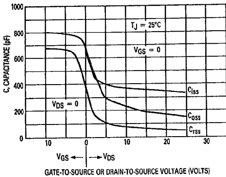
Figure 11. Capacitance Variation
