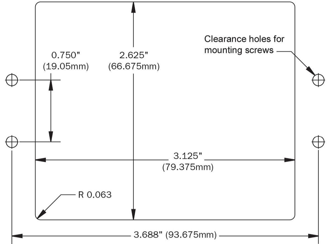
Flat Panel Mount Template
