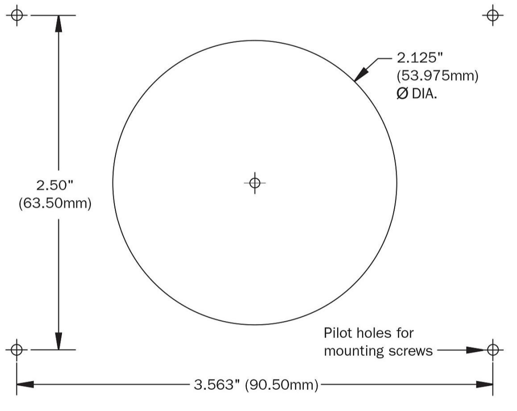
Surface Mount Template
